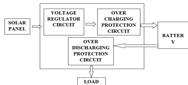
Figure:1. Block Diagram of Solar Charge Controller
