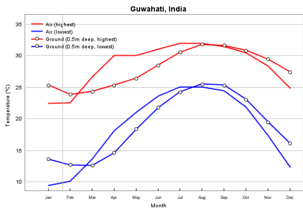
Fig.7: annual variation of temperature (highest and lowest) in air and 0.5m deep in the ground
