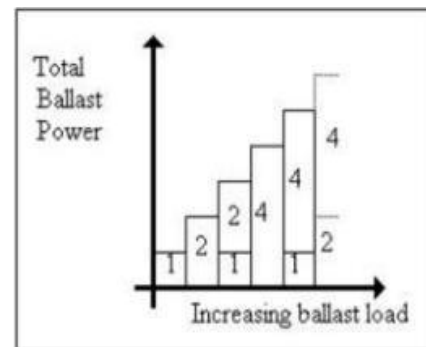
Fig. 1: Binary weighted ballast load [3].
